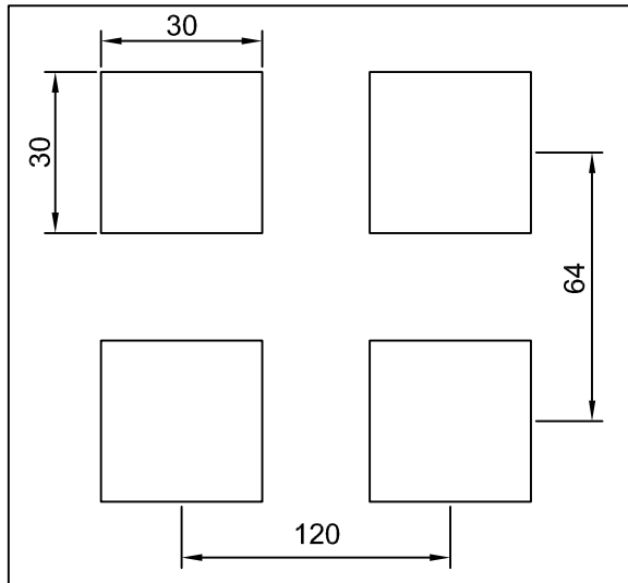
Fundamentplan Kicker Foosball
