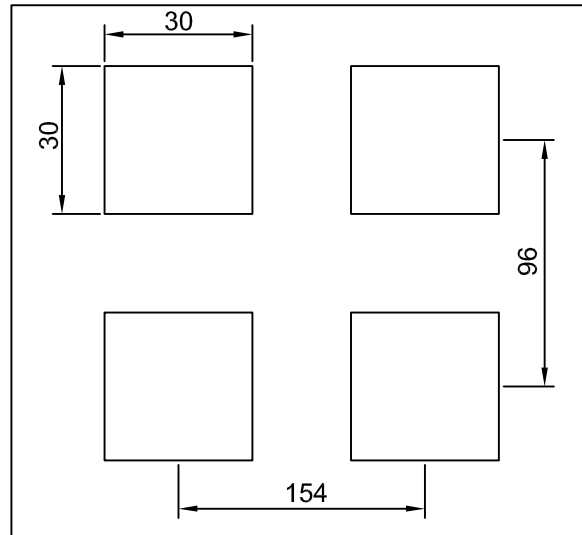
Fundamentplan Fero
